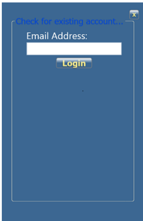
Figure 7 - Login screen
